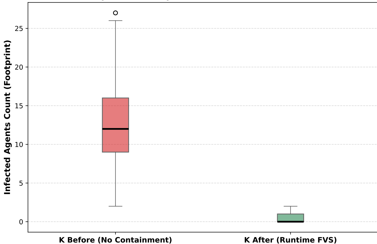
Compromise Footprint Before vs After Revocation
